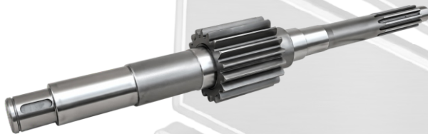
Part No. AG 110 Clutch Shaft 1312 (22" & 24") GDR
