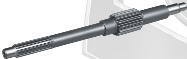
Part No. AG 145 Clutch Shaft PTL Type Preet 26.5"
